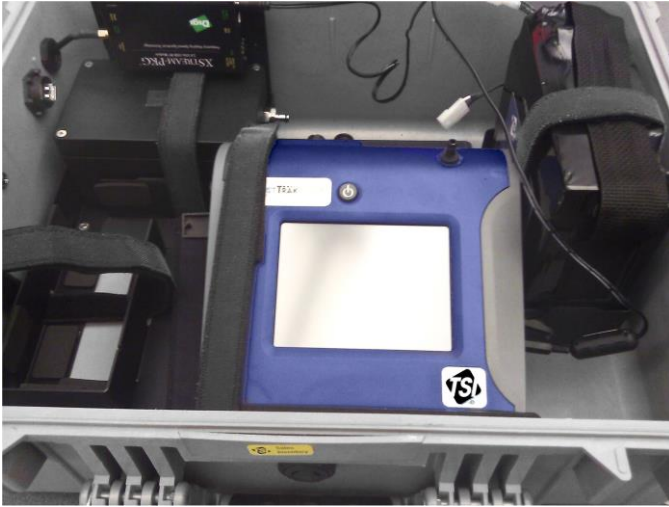
Figure 27: Install DustTrak Monitor in the Bracket
