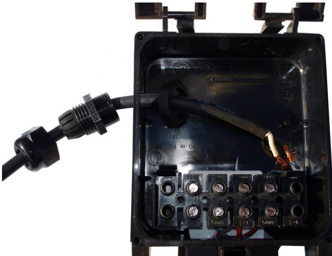
Figure 40: Strain Relief and Power Cable through Access Hole
