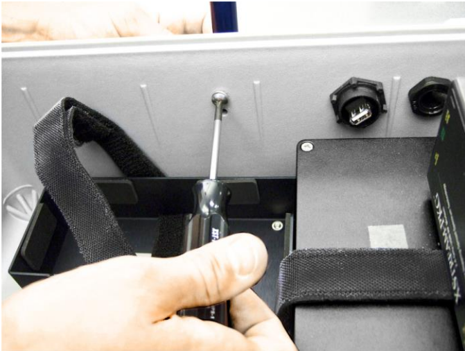
Figure 16: Attach Antenna Mounting Bracket to Enclosure
