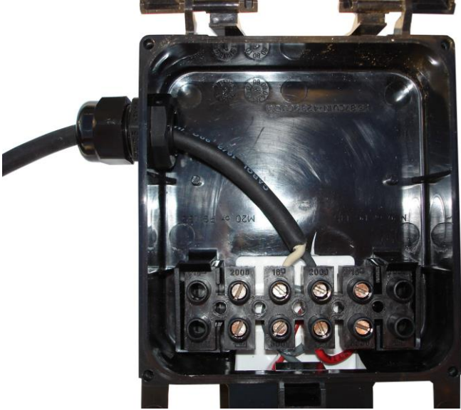
Figure 43: Secure Terminal Block and Tighten Strain Relief
